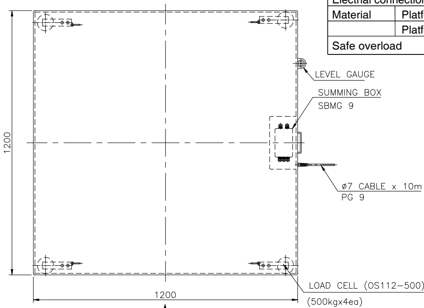
VIEW "A"
