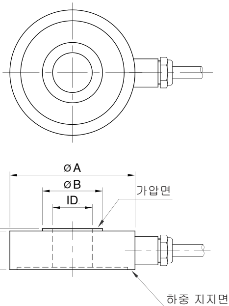
Dimension-mm
